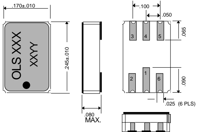
PACKAGE OUTLINE
