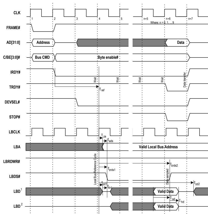
Figure 5: PCI Read Transaction from Motorola-type Local Bus
