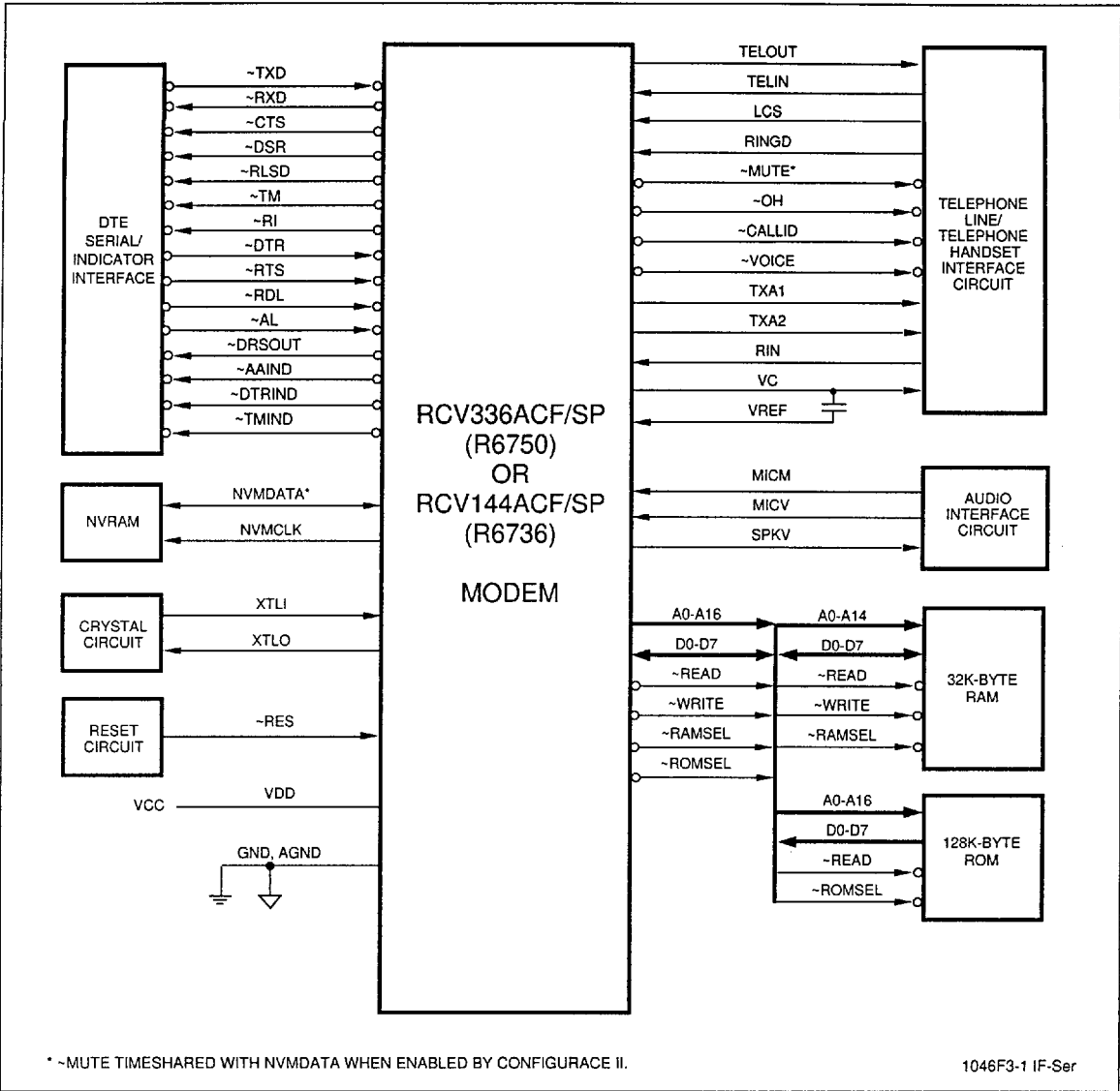
Figure 3-1. Hardware Interface Signals - Serial DTE Interface
