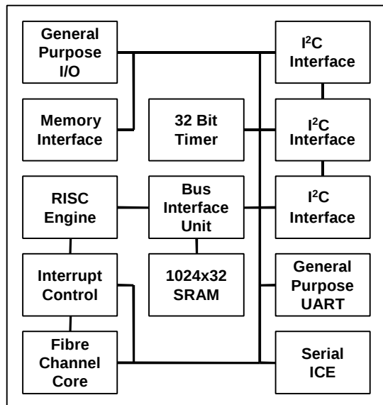
SSC100 Block Diagram
