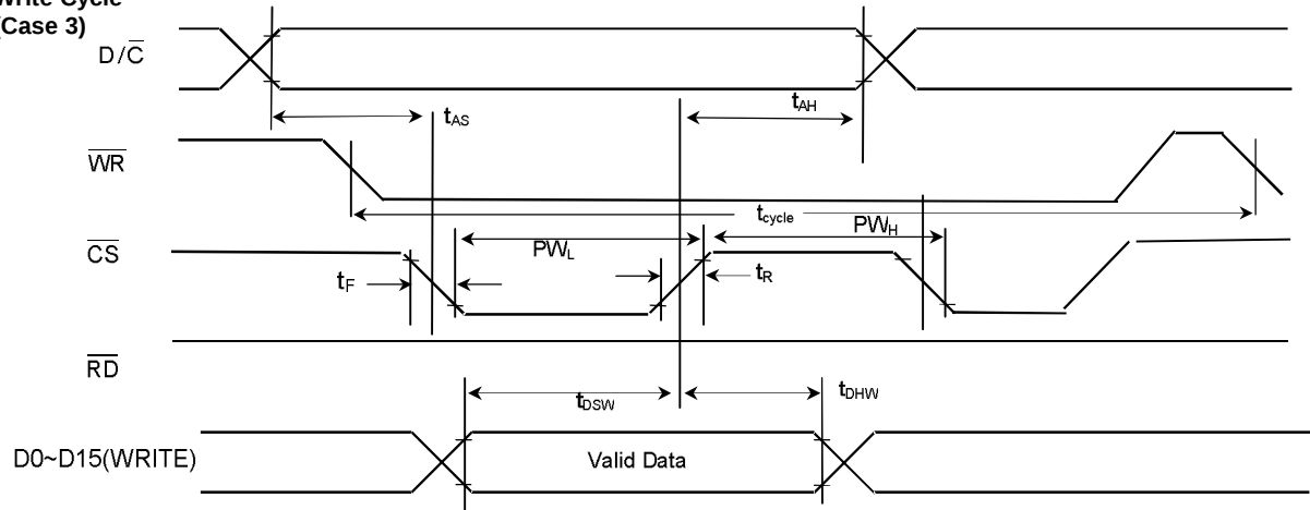
Write Cycle (Case 4)
