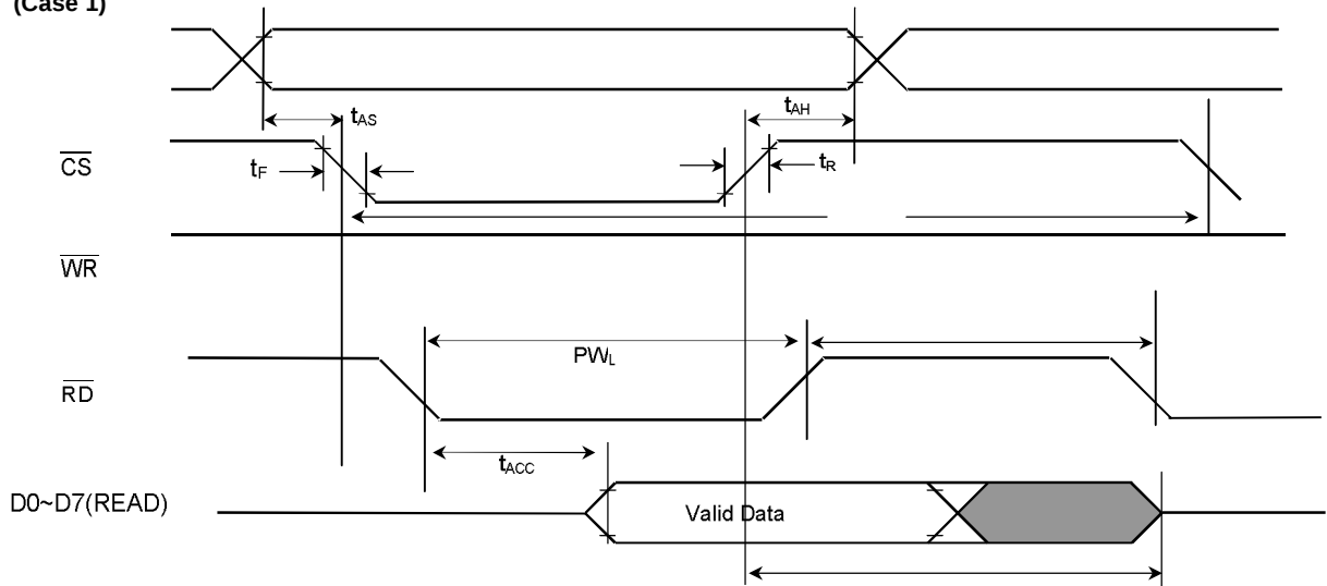
Read Cycle (Case 1)
