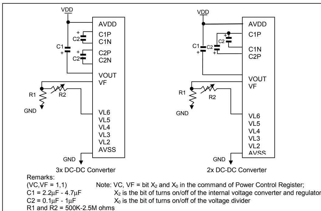
Figure 12 – When Built – in Power Supply is used
