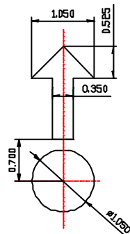
DETAIL D
