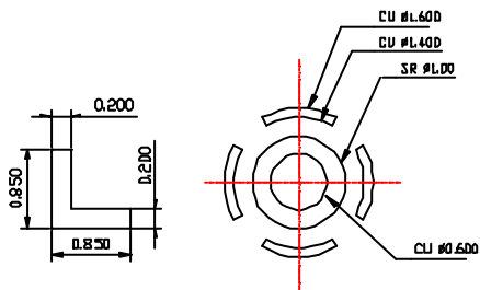
DETAIL C
