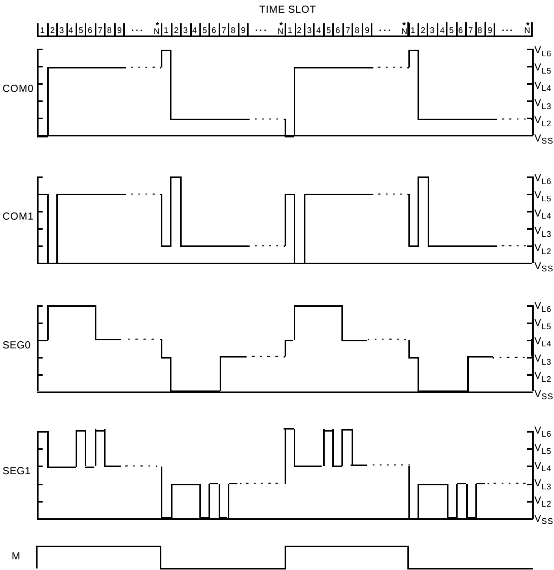
Figure 8a. LCD Display Example “0”
