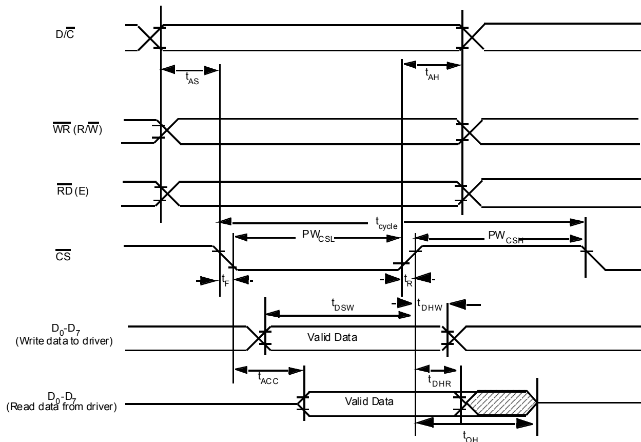
Figure 12 - Parallel 8080-series Interface Timing Characteristics ( \text{PS0} = \text{H} , \text{PS1} = \text{L} )
