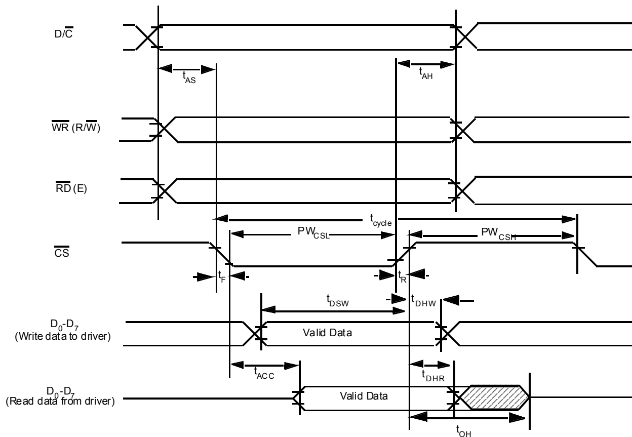
Figure 13 - Parallel 8080-series Interface Timing Characteristics ( \text{PS0} = \text{H} , \text{PS1} = \text{L} )
