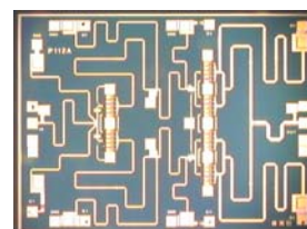
Dimension: 2.65mm x 2.0mm Thickness: 85um ± 15um
