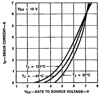
Figure 3 Transfer Characteristics
