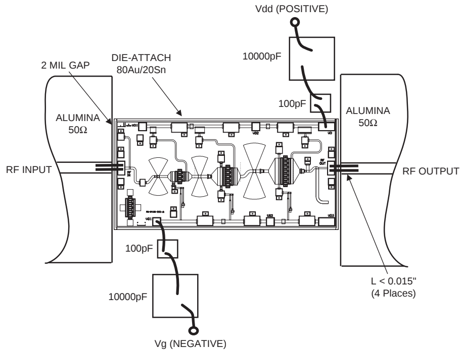
Figure 3. Recommended Application Schematic Circuit Diagram
