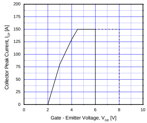
Fig 8. Collector Current Limit vs. Gate - Emitter Voltage Limit
