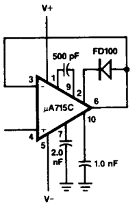
Voltage Follower (Note 1)
