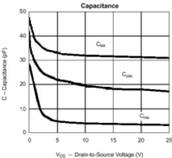
Figure 5. Capacitance
