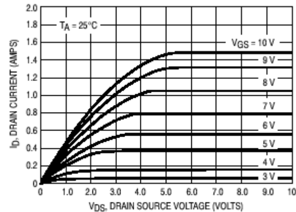
Figure 1. Ohmic Region
