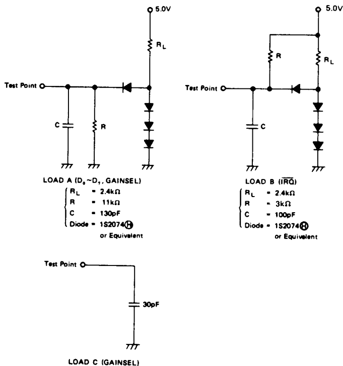
Figure 7 Test Load
