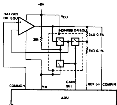
Figure 15 Pre-amplifier Circuit (x1, x4 Auto-Range Switching)
