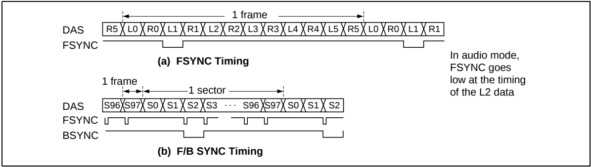
Figure 25 F/B SYNC Signal Timing Diagram
