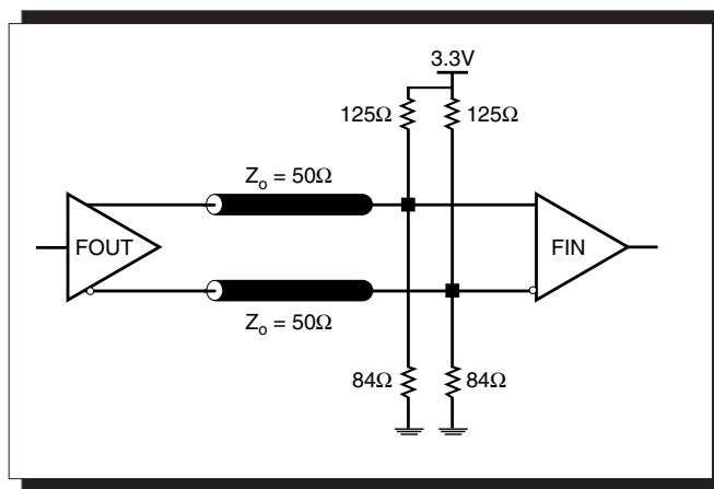
FIGURE 6B. LVPECL OUTPUT TERMINATION
