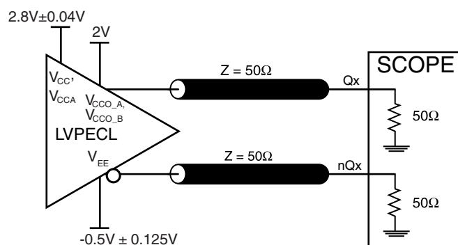
3.3V CORE/2.5V OUTPUT LOAD AC TEST CIRCUIT FOUTA0/nFOUTA0, FOUTB0/nFOUTB0
