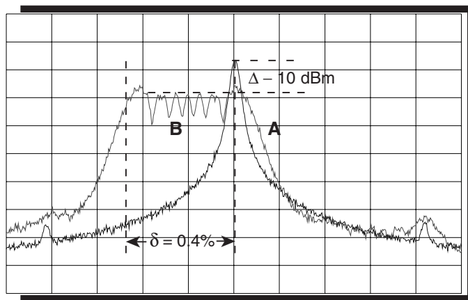
FIGURE 6B. 200MHz CLOCK OUTPUT IN FREQUENCY DOMAIN
