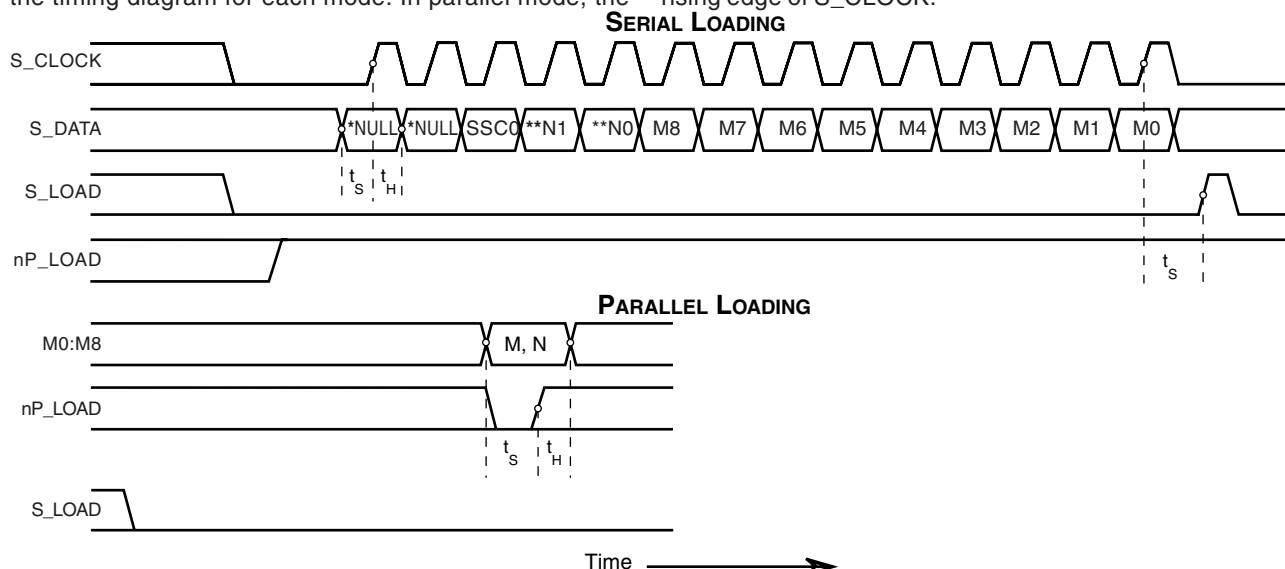
FIGURE 1. PARALLEL & SERIAL LOAD OPERATIONS
