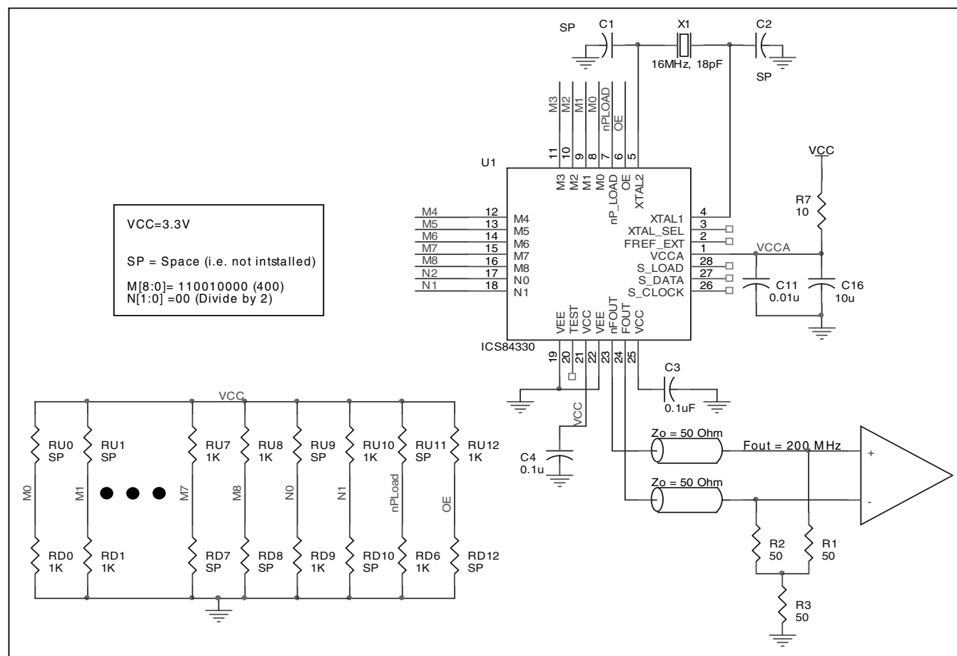
FIGURE 6A. SCHEMATIC OF RECOMMENDED LAYOUT
