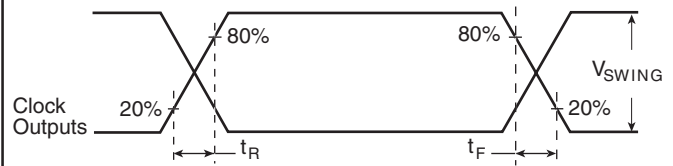
PROPAGATION DELAY
