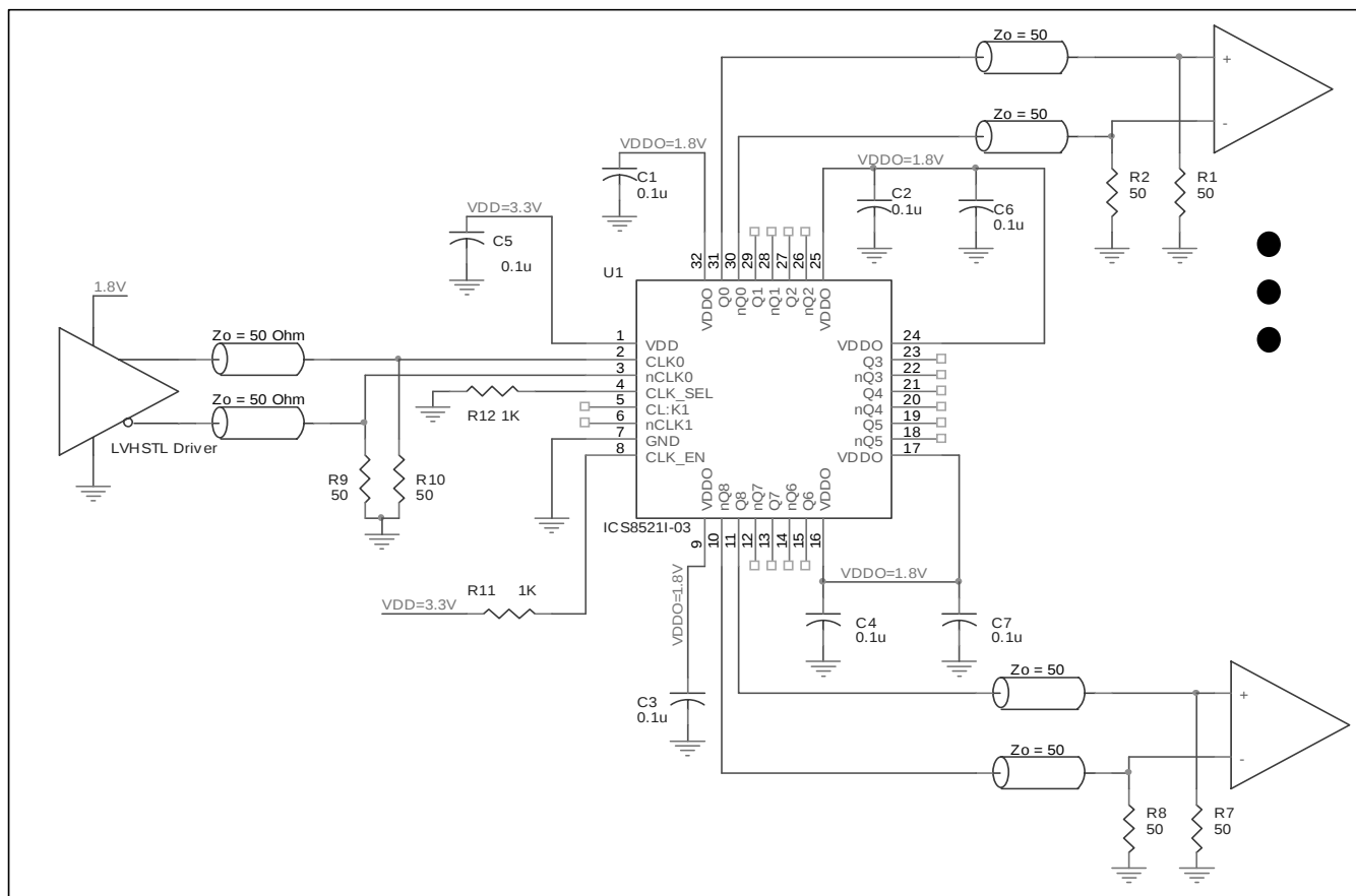
FIGURE 3B. RECOMMENDED LAYOUT OF BYPASS CAPACITOR PLACEMENT
