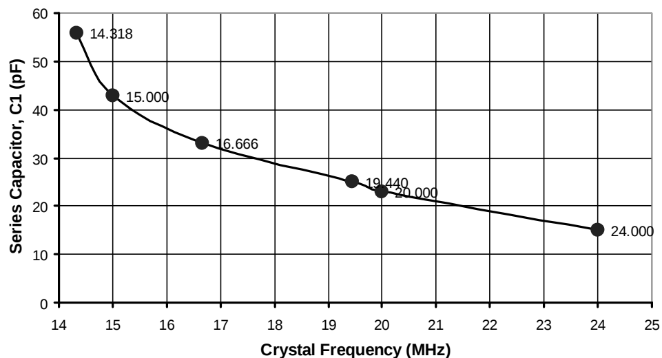
FIGURE 8 - SUGGESTED SERIES CAPACITOR C1 FOR PARALLEL CRYSTAL
