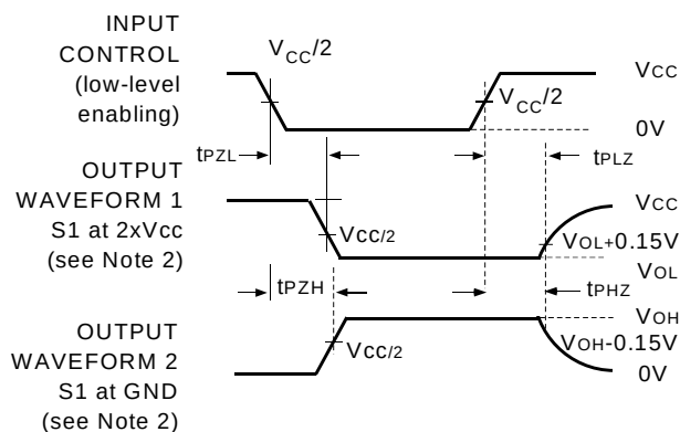
Voltage Waveforms Enable and Disable Times
