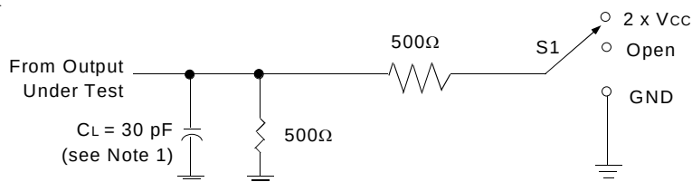
Load Circuit
