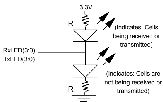
Figure 31 LED Indicator
