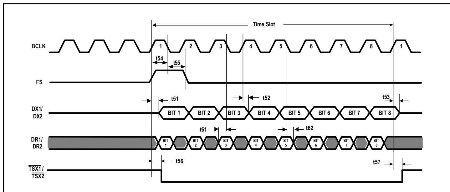
Figure 16. Transmit and Receive Timing *
