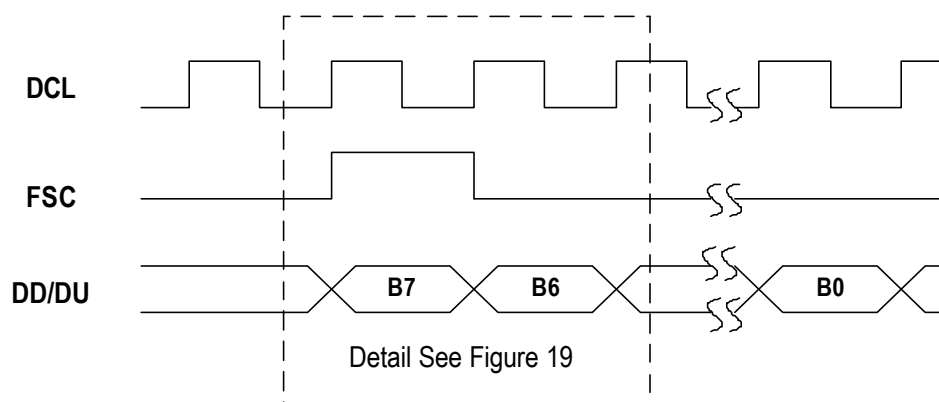
Figure 18. GCI Interface Timing
