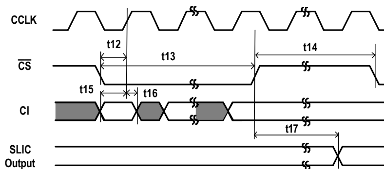
Figure 14. MPI Input Timing
