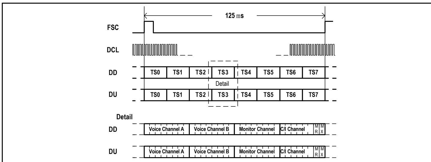
Figure 4. Compressed GCI Frame Structure
