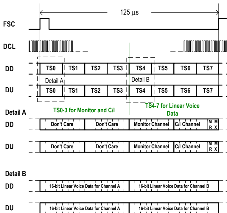
Figure 5. Linear GCI Frame Structure When TS Is Low
