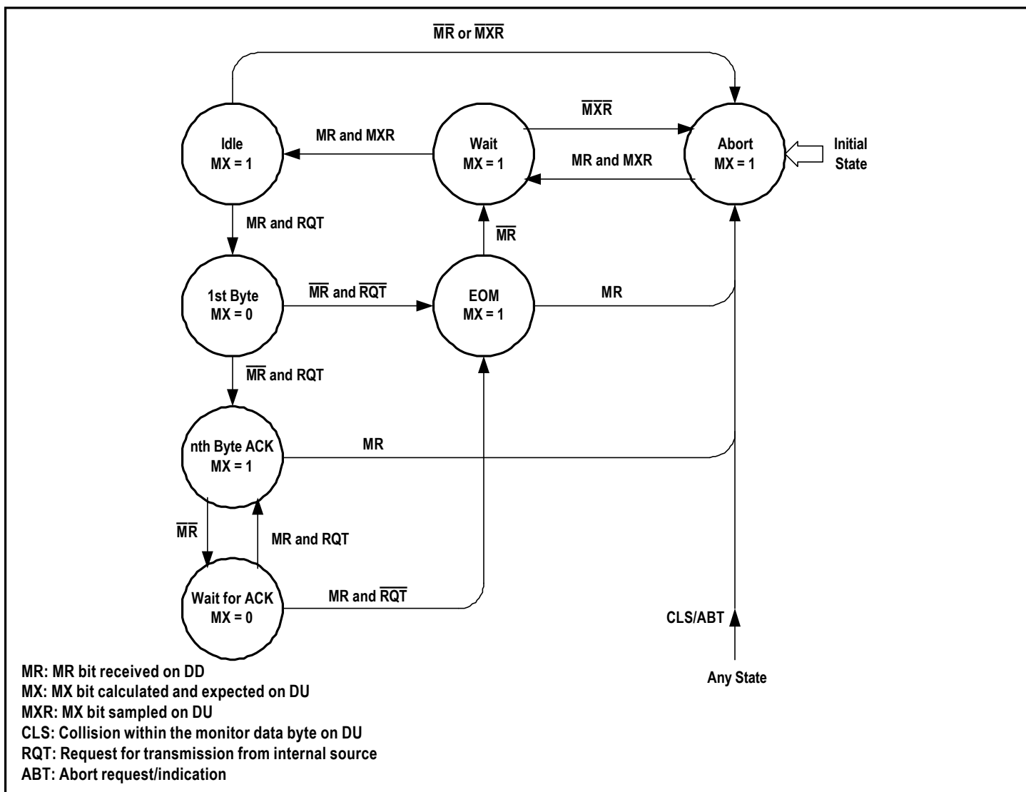
Figure 7. State Diagram of Monitor Transmitter
