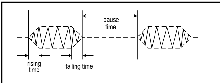
Figure 12. Teletax Signal
