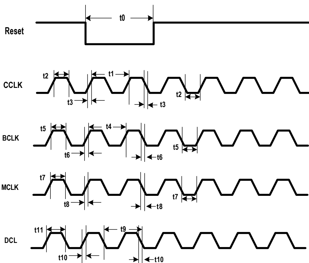
Figure 13. Reset and Clock Timing
