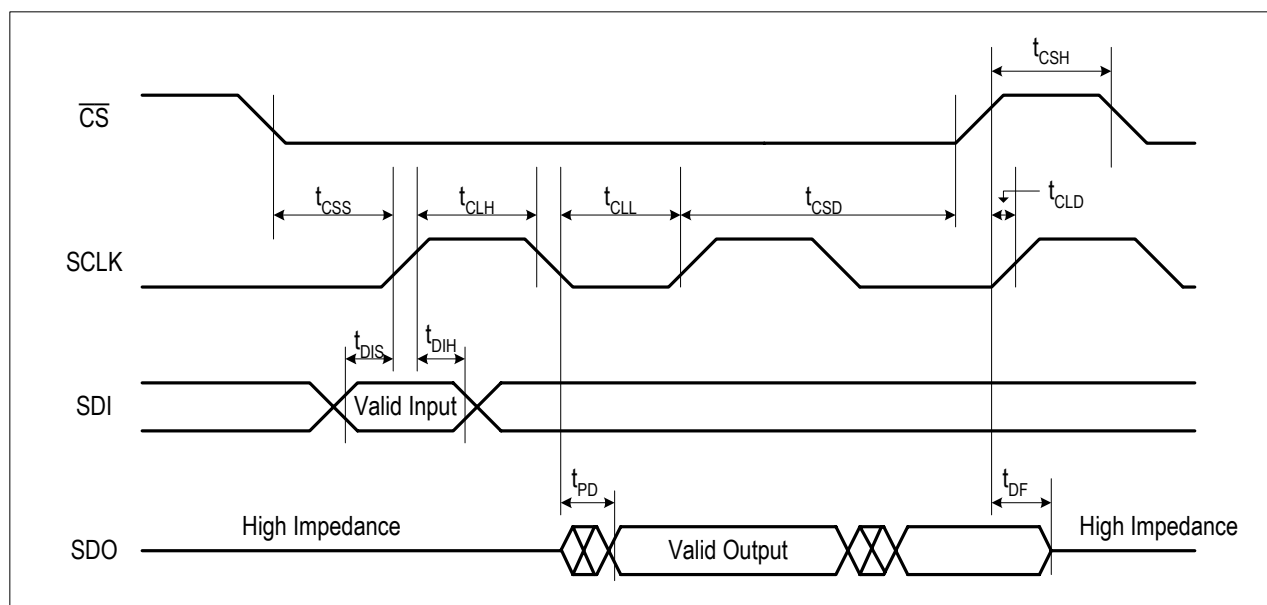
Figure 51. SPI Timing Diagram
