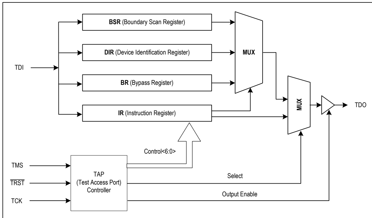
Figure 39. JTAG Architecture
