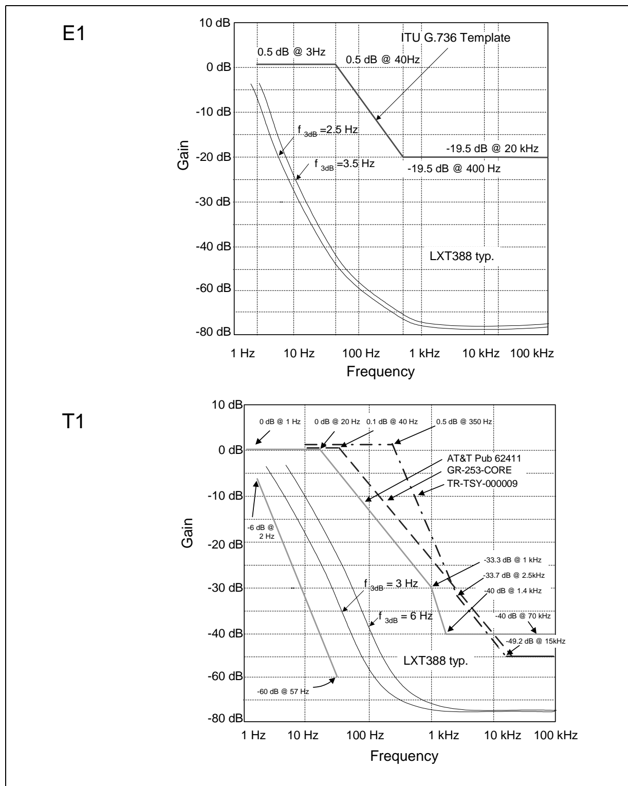
Figure 35. Jitter Transfer Performance
