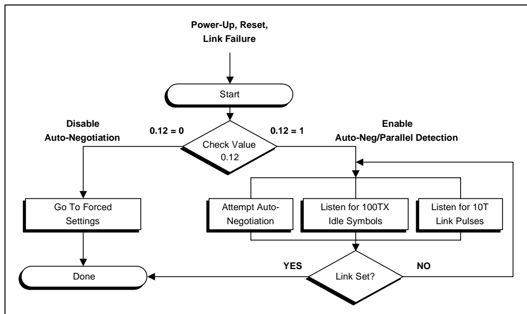
Figure 8. Auto-Negotiation Operation
