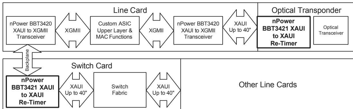
FIGURE 1. BBT3421 APPLICATIONS
