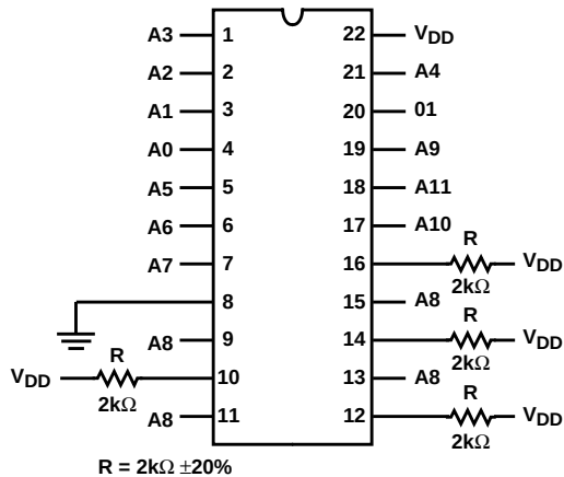
FIGURE 5. DYNAMIC/OPERATING BURN-IN CIRCUIT AND TIMING DIAGRAM
