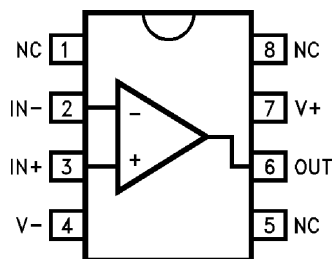
EL2075 (8-PIN SO, PDIP) TOP VIEW
