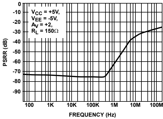
FIGURE 12. PSRR ( V_{CC} )
