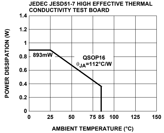
FIGURE 15. PACKAGE POWER DISSIPATION vs AMBIENT TEMPERATURE
