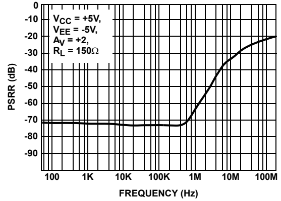
FIGURE 13. PSRR ( V_{EE} )
