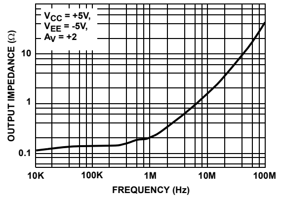
FIGURE 7. CLOSED LOOP OUTPUT IMPEDANCE
