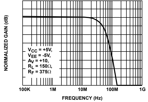
FIGURE 3. FREQUENCY RESPONSE FOR A_V = +10
