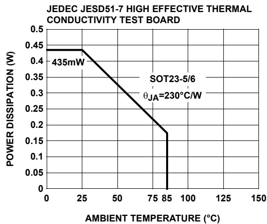
FIGURE 16. PACKAGE POWER DISSIPATION vs AMBIENT TEMPERATURE
