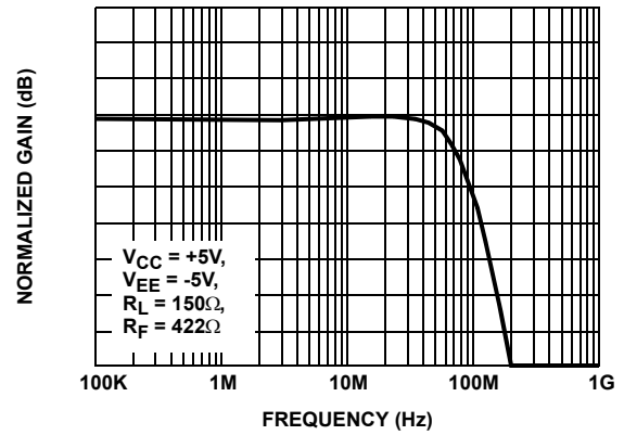
FIGURE 5. FREQUENCY RESPONSE FOR A_V = +4
