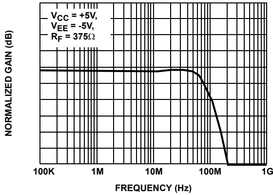
FIGURE 2A. FREQUENCY RESPONSE FOR A_V = +4.6
