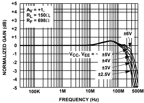
FIGURE 6. FREQUENCY RESPONSE FOR VARIOUS V_{CC} , V_{EE}
