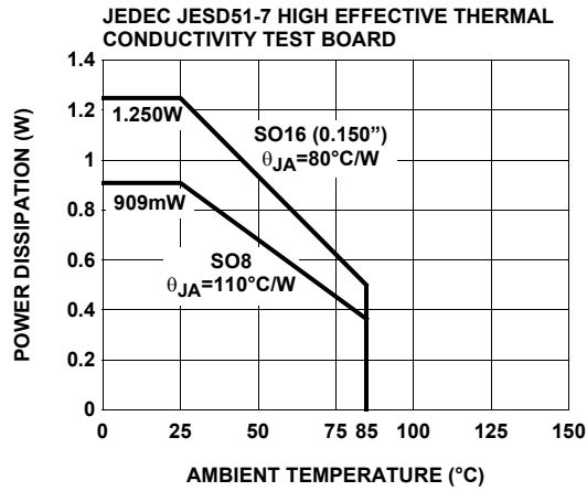
FIGURE 14. PACKAGE POWER DISSIPATION vs AMBIENT TEMPERATURE
