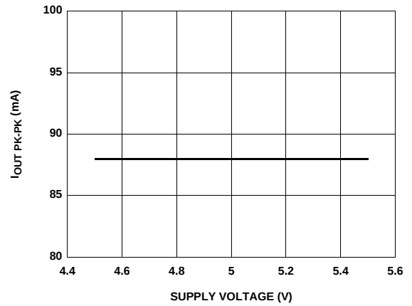
FIGURE 10. PEAK-TO-PEAK OUTPUT CURRENT vs SUPPLY VOLTAGE
