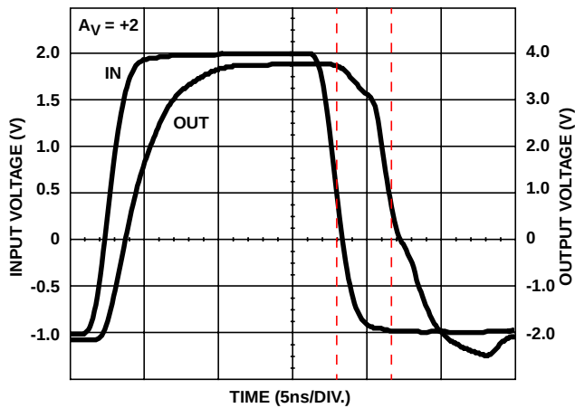
FIGURE 4. PULSE RESPONSE WITHOUT LIMITING
