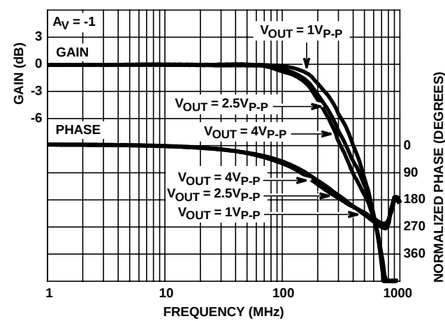
FIGURE 21. FREQUENCY RESPONSE FOR VARIOUS OUTPUT VOLTAGES
