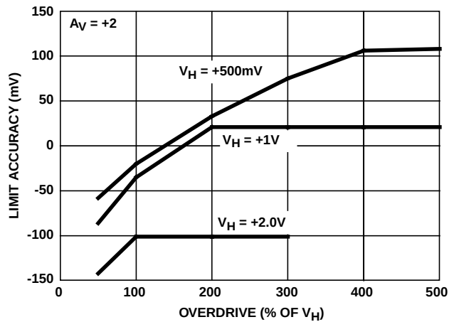
FIGURE 28. V_H LIMIT ACCURACY vs OVERDRIVE
