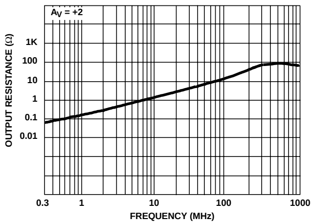
FIGURE 26. OUTPUT RESISTANCE
