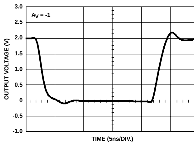
FIGURE 15. LARGE SIGNAL POSITIVE PULSE RESPONSE
