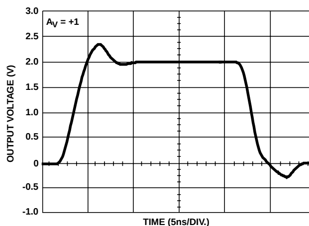
FIGURE 11. LARGE SIGNAL POSITIVE PULSE RESPONSE
