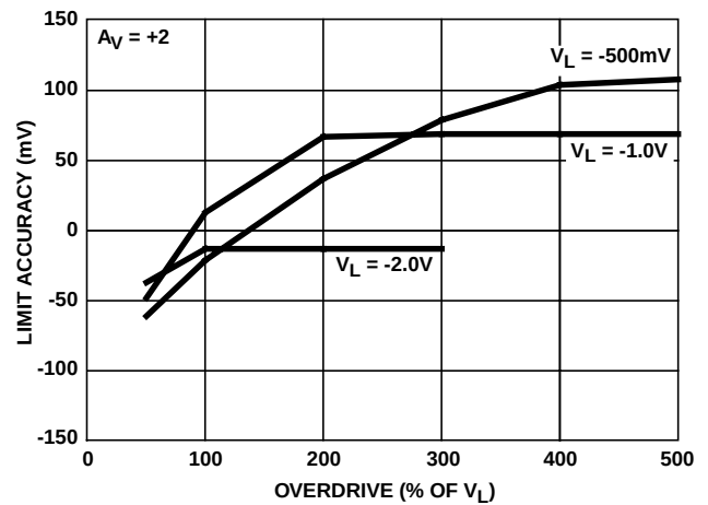
FIGURE 29. V_L LIMIT ACCURACY vs OVERDRIVE
