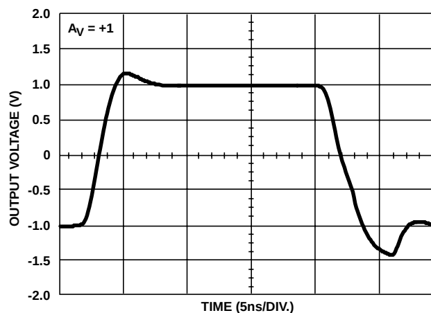
FIGURE 13. LARGE SIGNAL BIPOLAR PULSE RESPONSE
