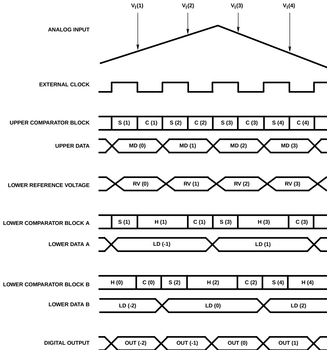
FIGURE 5. TIMING CHART 2
