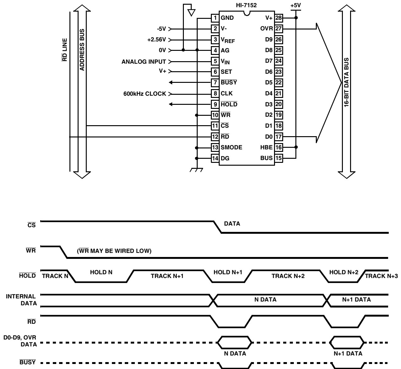
FIGURE 6. FAST MEMORY MODE APPLICATION
