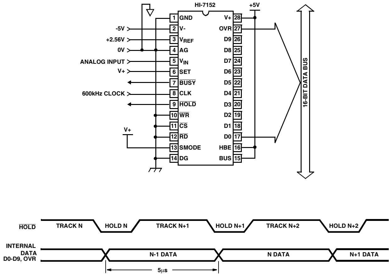
FIGURE 7. DMA MODE APPLICATION
