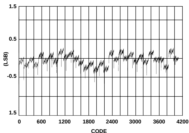
FIGURE 6. TYPICAL INL
