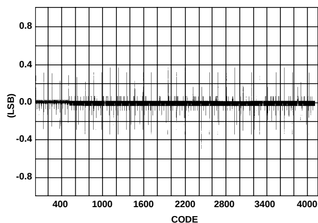
FIGURE 7. TYPICAL DNL
