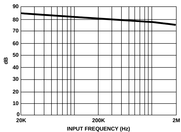
FIGURE 5. TYPICAL THD vs INPUT FREQUENCY
