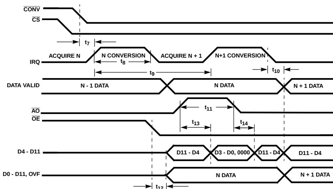
FIGURE 3. CONTINUOUS CONVERSION TIMING
