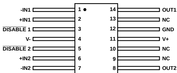
HS-1254RH (FLATPACK) TOP VIEW
