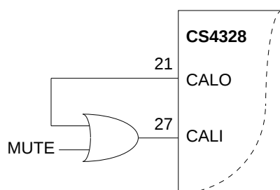
Figure 7. -50dB Muting
