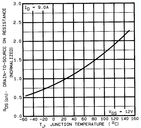
Fig 21. Normalized On-Resistance Vs. Temperature
