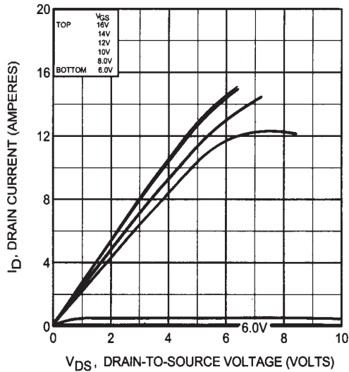
Fig 10. Typical Output Characteristics Pre-Irradiation
