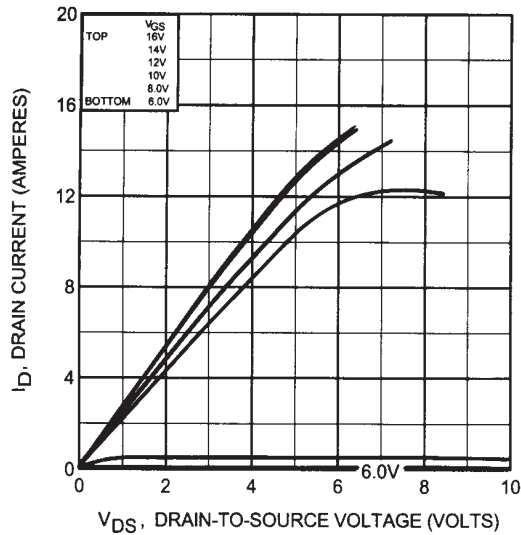
Fig 14. Typical Output Characteristics Pre-Irradiation
