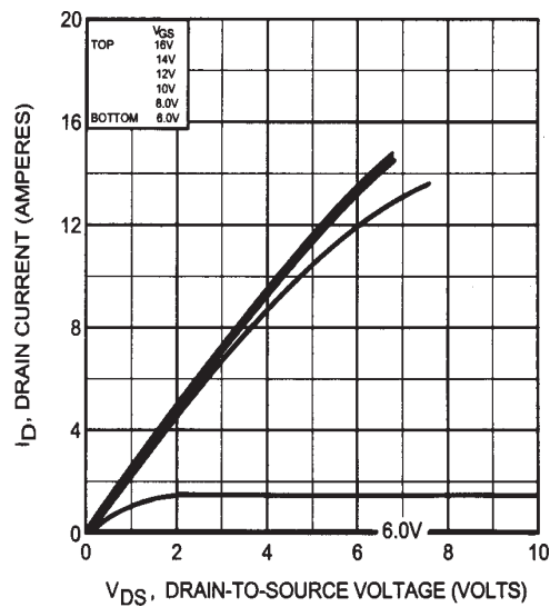
Fig 12. Typical Output Characteristics Post-Irradiation 300K Rads (Si)
