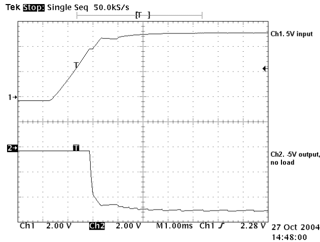
Figure. 13 Start up
