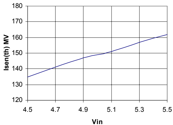
Current comparator threshold versus V_{in} ( T_A=25^\circ\text{C} )
