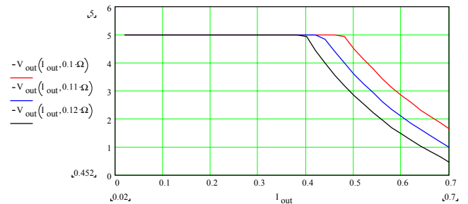
Figure 22 - Theoretical output voltage versus output current with different current sensing resistor R_s .
