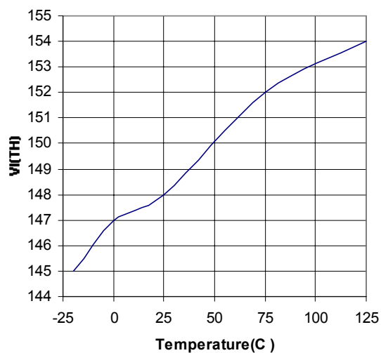
Figure. 10. Current sensing comparator upper threshold versus temperature ( V_{CC}=5\text{V} )
