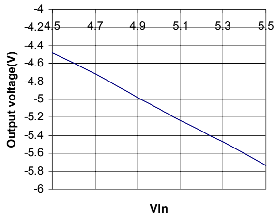
Output voltage versus V_{in}@I_{out}=200\text{mA} , T_A=25^\circ\text{C}
