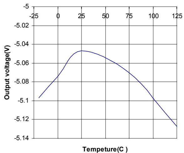
Output voltage versus temperature ( V_{in}=5\text{V} , I_{out}=200\text{mA} )
