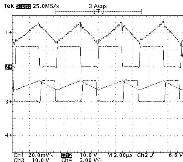
Figure 17 - Normal condition at 15A. Ch1: Output Voltage Ripple (20mV/div) Ch2: HDrv Ch3: LDrv Ch4: Inductor Current (5A/div)
