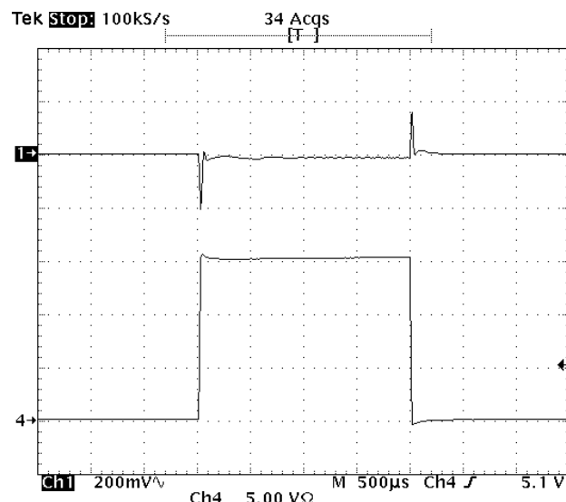
Figure 16 - Transient load response at I_{OUT}=0A - 15A . Ch1: V_{OUT} Ch4: I_{OUT} (5A/div)
