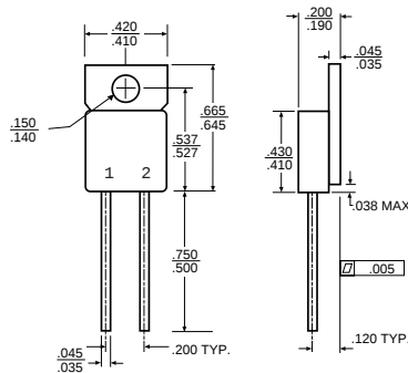
T0-257AA 2-Pin
