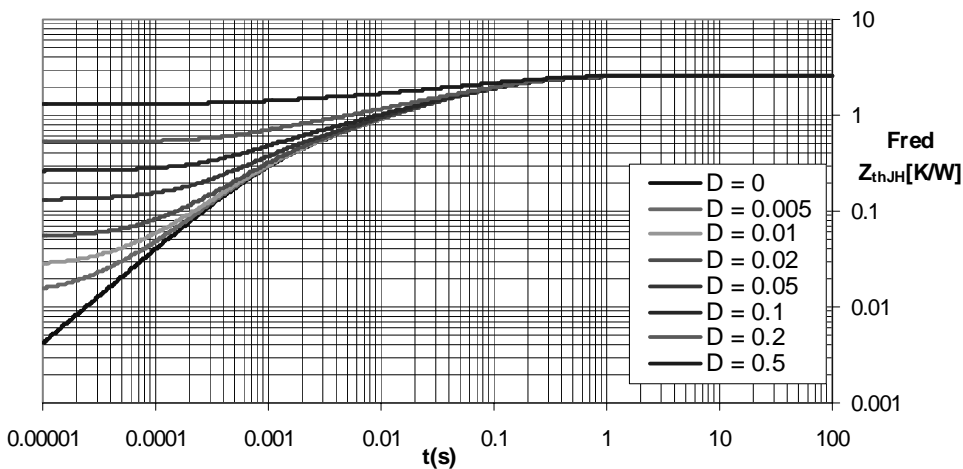
Transient thermal resistance junction to heatsink
