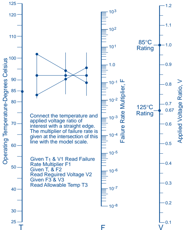
Figure 12. Reliability Nomograph
