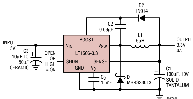
5V to 3.3V Down Converter
