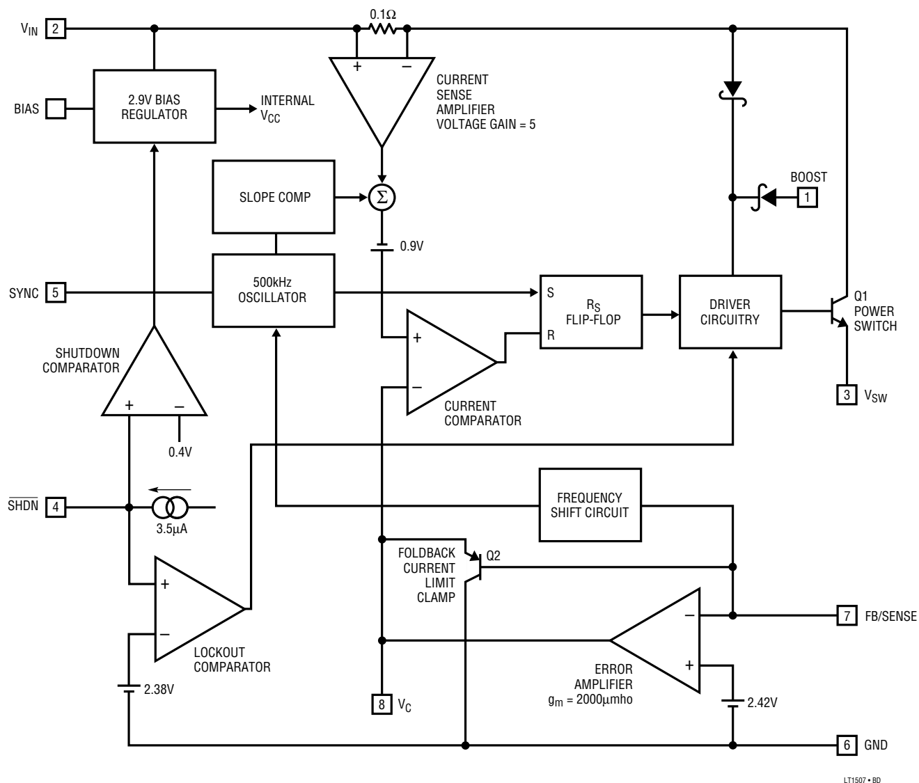
Figure 1. Block Diagram
