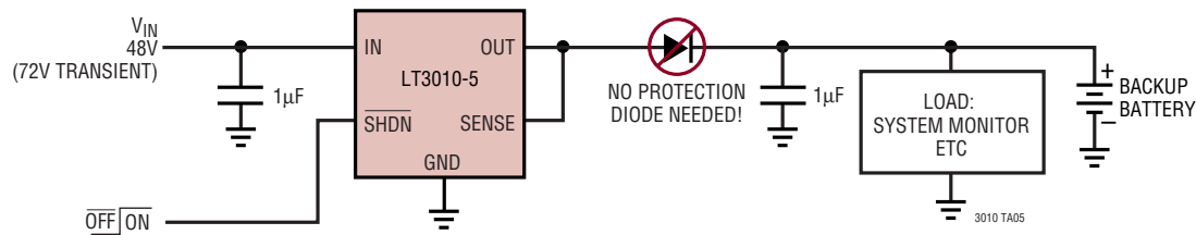
LT3010 Telecom Application
